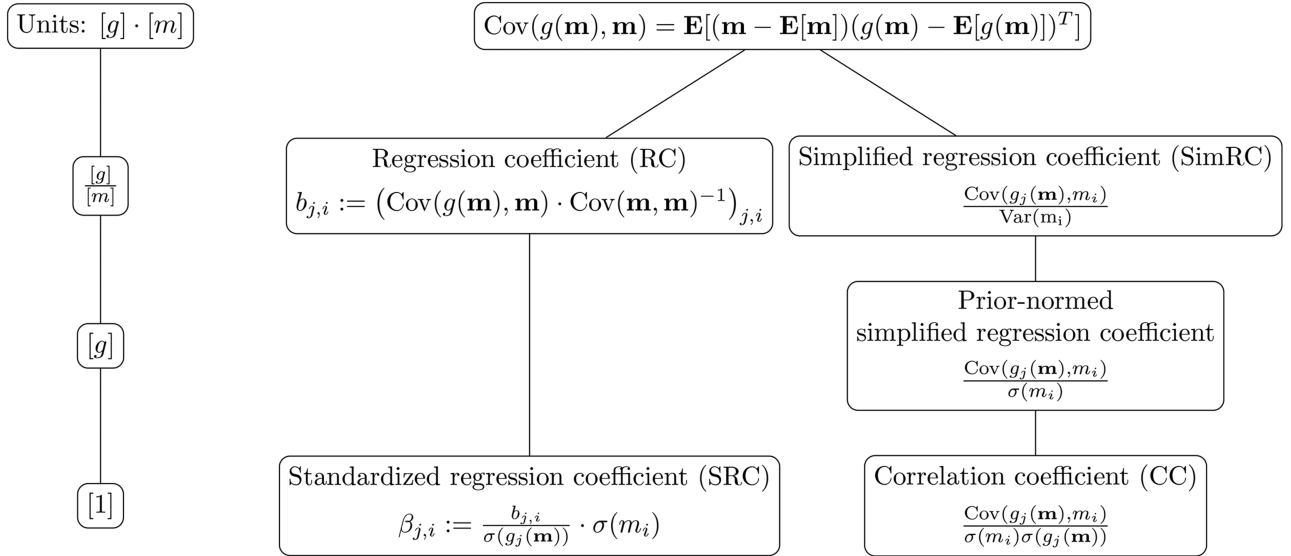
Figure 1 Sensitivity measure candidates derived from the full prior distribution \rho(\mathbf{m}) and forward model g ; E is the expectation operator with respect to \rho(\mathbf{m}) ; RC and SRC as used by Saltelli et al. (2004).
